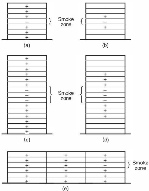
FIGURE A.4.8.1.1 Arrangements of Smoke Control Zones.
