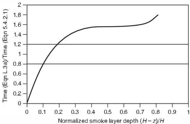
FIGURE L.3(b) Comparison of Algebraic Equations, Equations 5.4.2.1a or 5.4.2.1b and L.3a: Steady Fire — Normalized Smoke Layer Depth.
