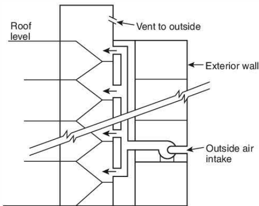
FIGURE E.4 Stairwell Pressurization with Vent to the Outside.
